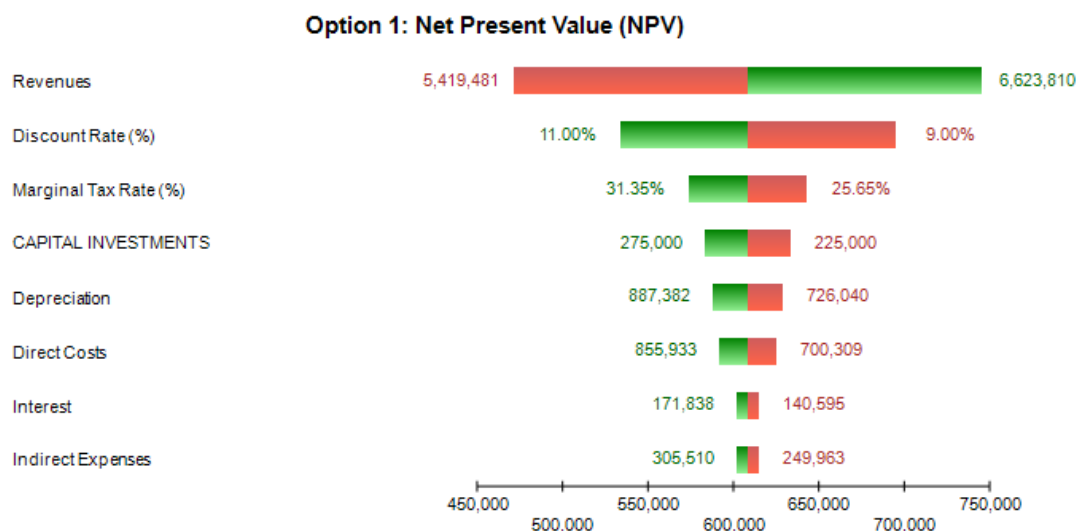
Figure 12: Applied Analytics—Tornado Analysis
